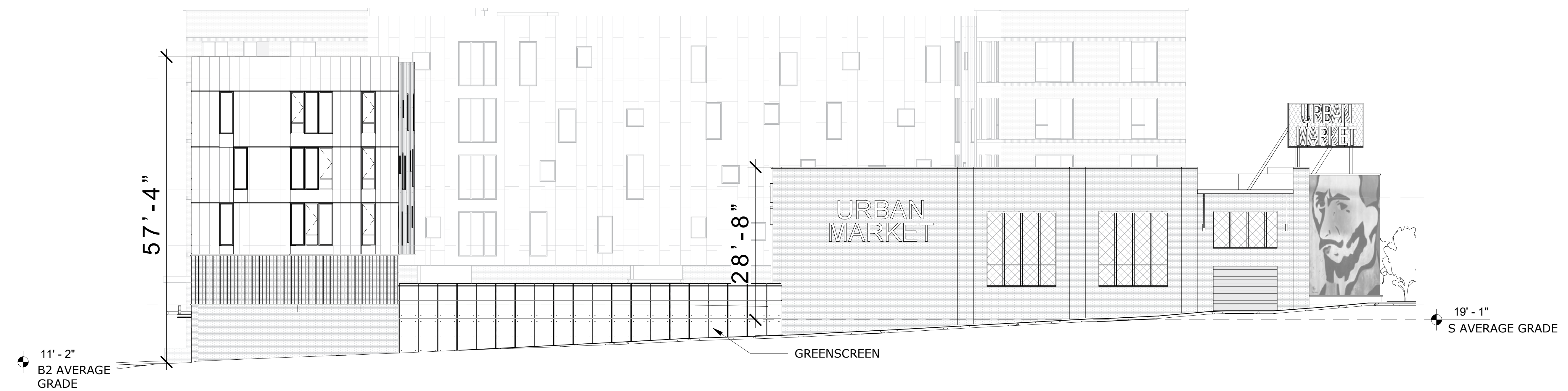
PIKE STREET ELEVATION
