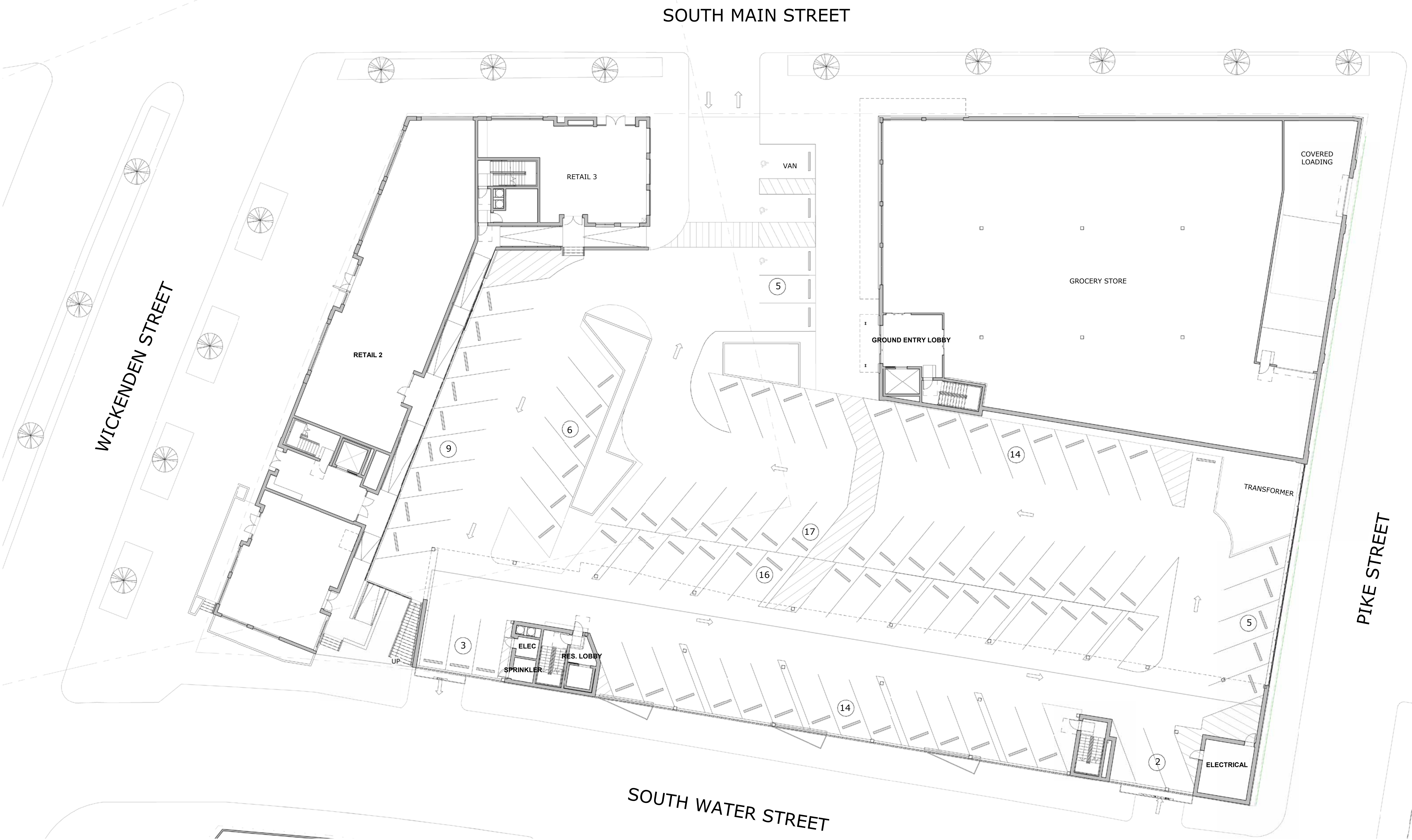
GROUND FLOOR PLAN (91 PARKING SPACES)
